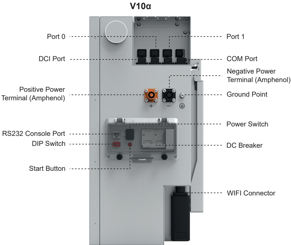
Figure 3-2 Appearance component name
